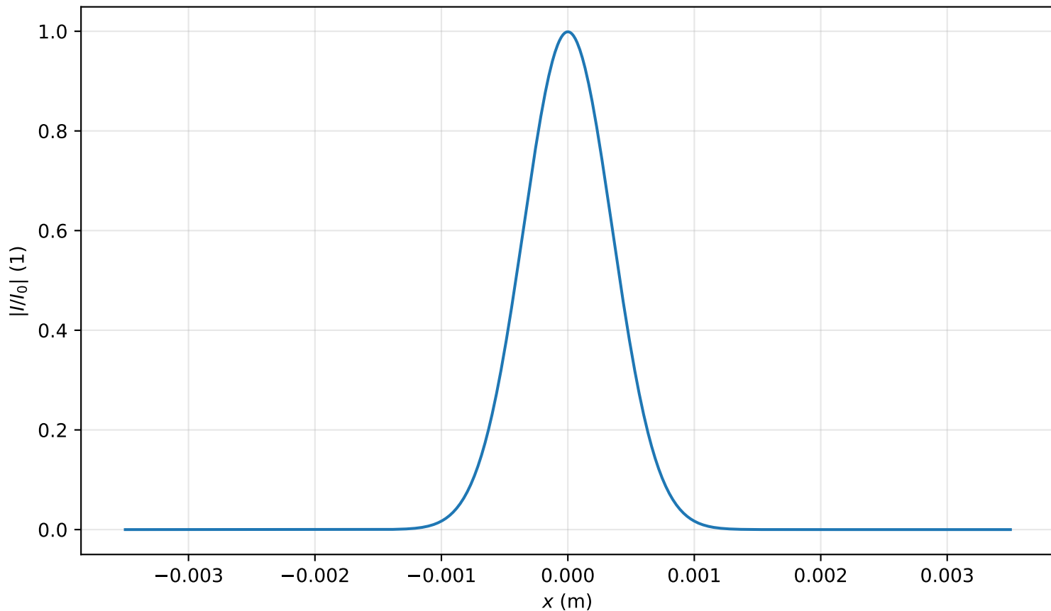
Intensity profile I(x, y = 0, z = 0.080m)/I_0 , P_{in}=0.1P_{cr} , artificial time
